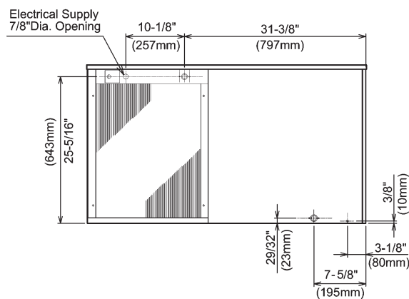
AIR-COOLED UNIT
